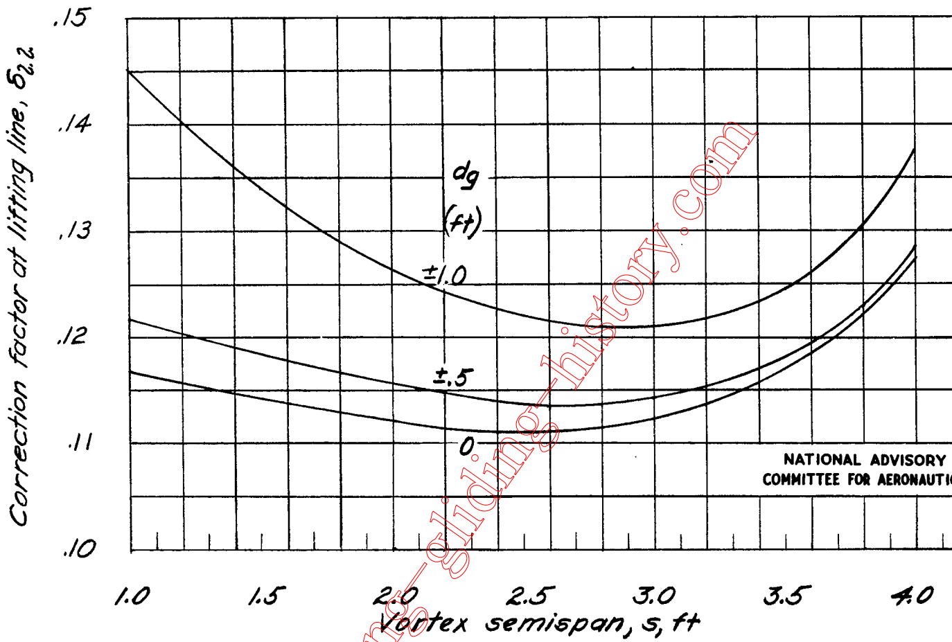
Figure 6.- Correction factor at the lifting line in 7-by 10-foot closed rectangular wind tunnels.
